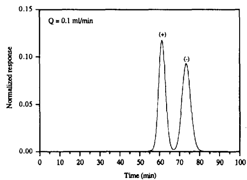
Fig. 1. Effect of flow-rate on enantiomer separation with column A (25 cm \times 0.46 cm I.D.) packed with TCA particles of d_p = 15\text{--}25\ \mu\text{m} .
